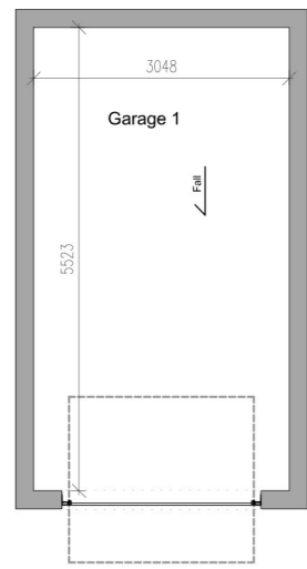
FLOOR PLAN
